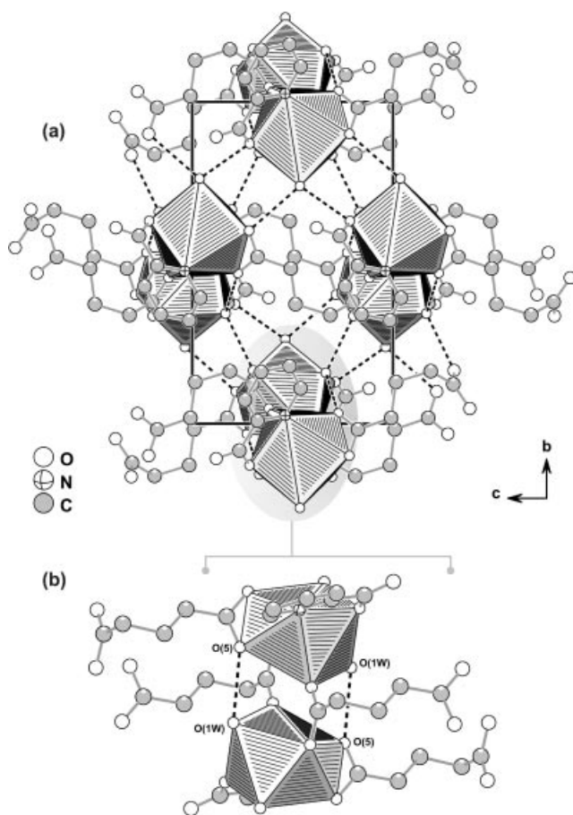
Figure 2. (a) Crystal packing of [Sm(glu)(pic)(H 2 O) 2 ] viewed along the [100] direction of the unit cell. (b) Intra-dimer hydrogen bonds involving the coordinated O(1) water molecule and the syn,syn chelating carboxylato group. Hydrogen atoms and symmetry codes used to generate equivalent atoms have been omitted for clarity. Hydrogen bonds are represented as black-filled dashed lines. For hydrogen bonding geometric details see Table 2.
