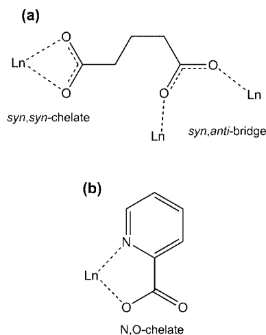
Scheme 1. Coordination modes of the ligands present in [Sm(glu)(pic)(H 2 O) 2 ]: (a) glutaric acid; (b) picolinic acid.
